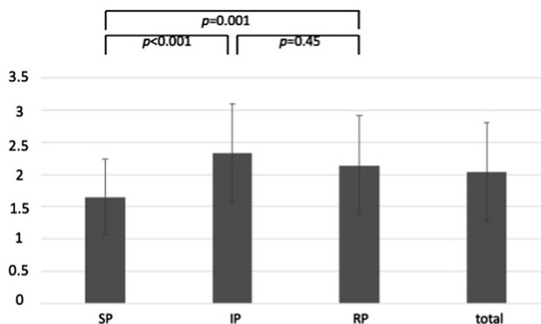
Fig. 1 External assessment using the CARE-Scale (SP = simulated-patient-group; IP = incognito-patient-group; RP = real-patient-group). Y-axis displays CARE-Scale rating. Data are presented as mean + standard deviation
